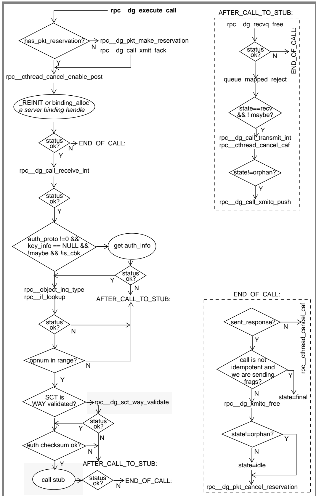
Figure 7-17: Call Execution
