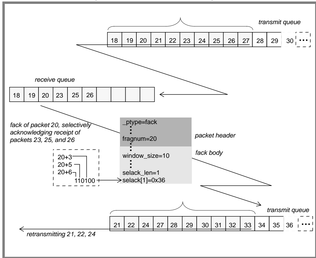
Figure 6-7: Selective Acknowledgment
