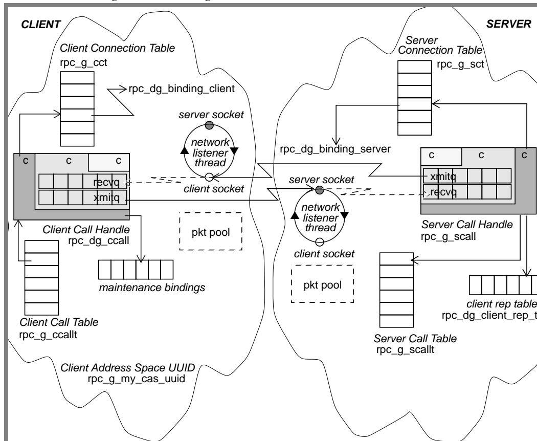
Figure 6-1: Datagram RPC Protocol Service Elements
