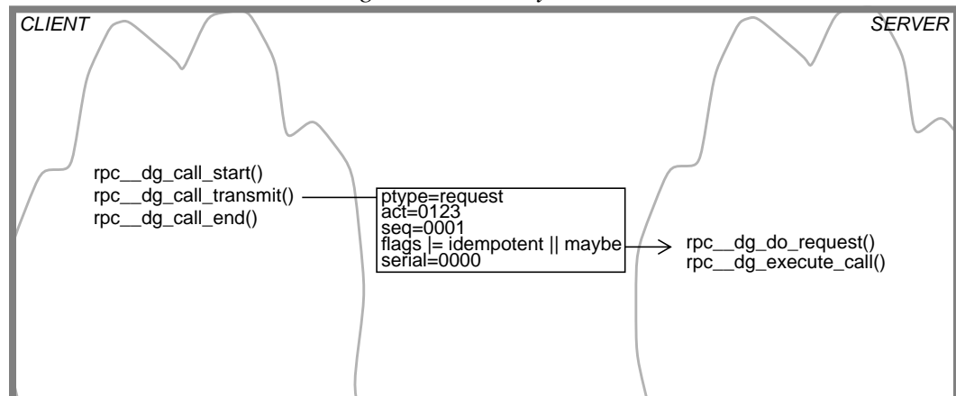
Figure 7-4: A Maybe Call
